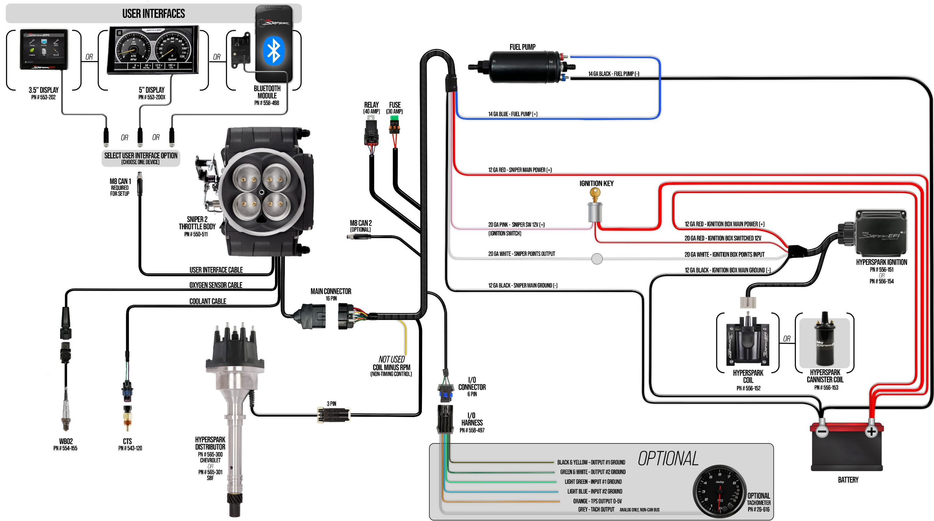
DIAGRAM 3: SNIPER 2 ECO SYSTEM WITHOUT USING A SNIPER EFI PDM
