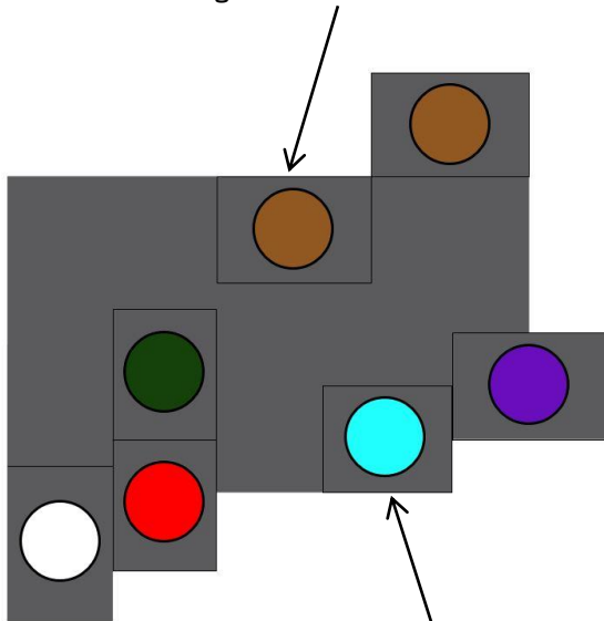
Figure 9 – End View (Harness Side) Late 1965 to 1966 Corvette
