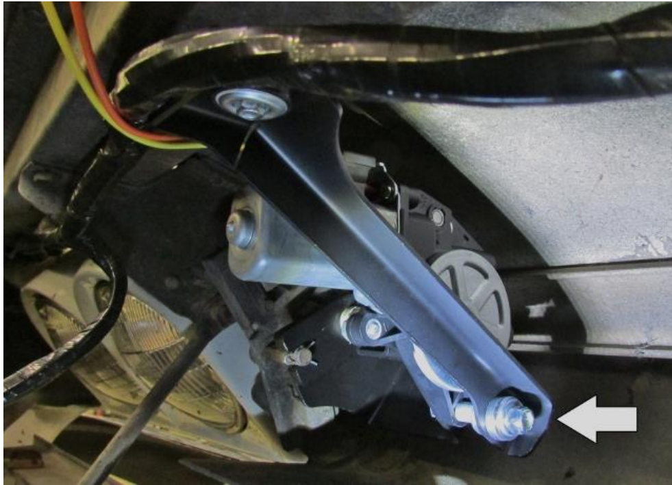
Figure 6 – Tighten Support Bracket
